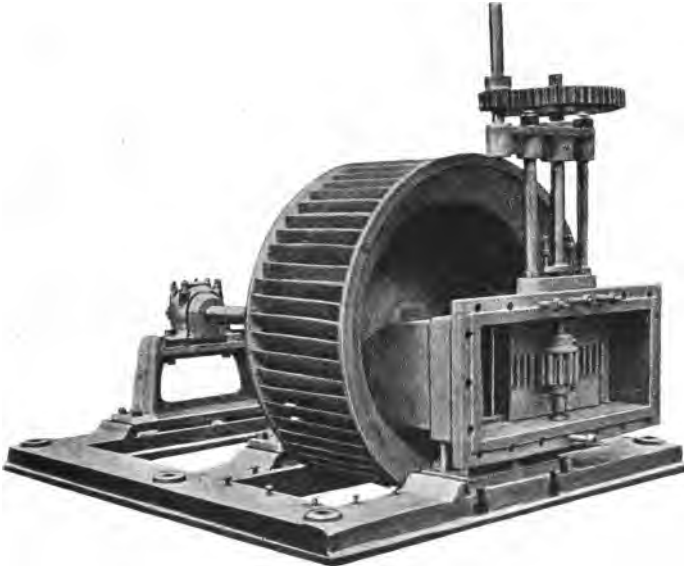
Fig. 50. Schwammkrug-Turbine.
